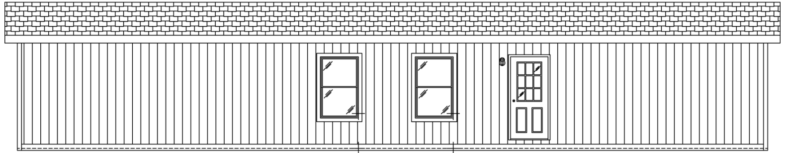
REAR SIDEWALL
